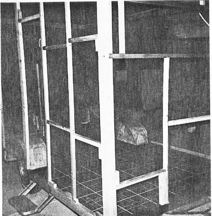
COAX TRAILER SHOWING NEW FRAME STRUCTURE VIEW 1
